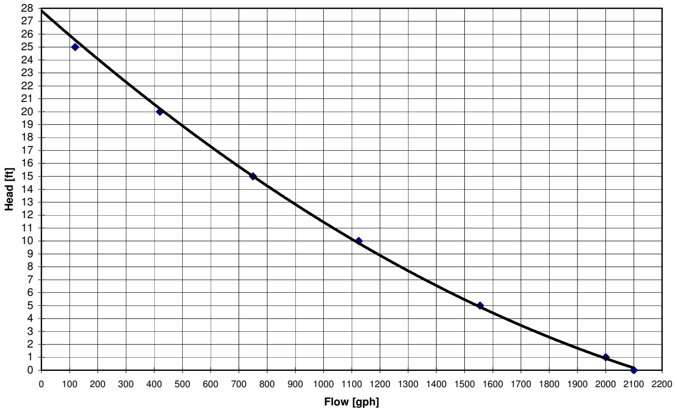
PW2000 Pump Curve Waterfall pump
